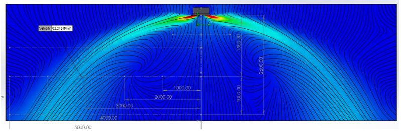
LP-12"-300cfm
