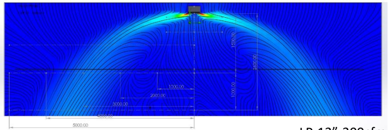
LP-12"-300cfm
